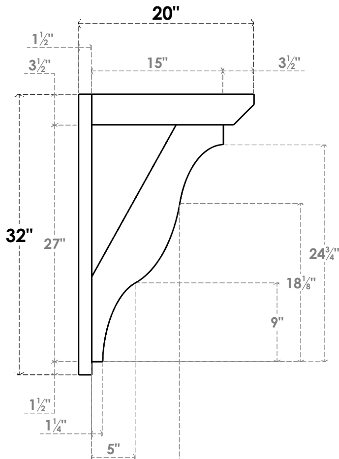
SIDE PROFILE
